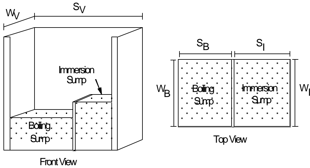
Figure 307-4. Solvent Cleaner Dimensions.
